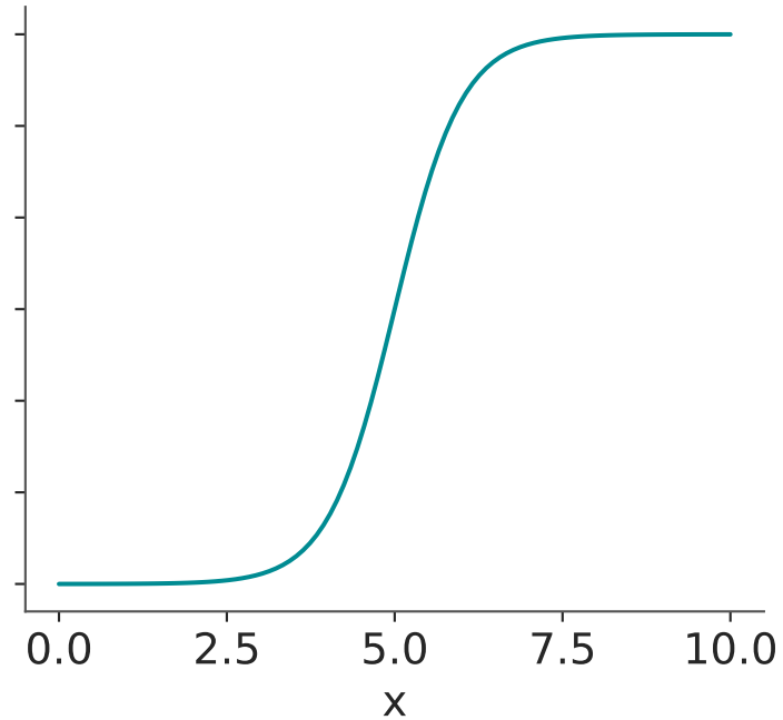
Sigma = 1.5
