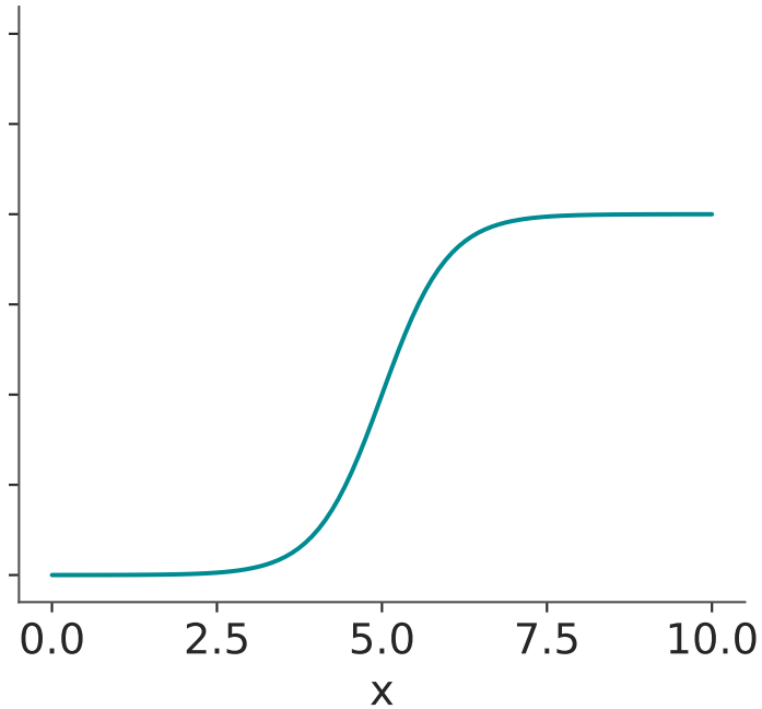
Sigma = 1
