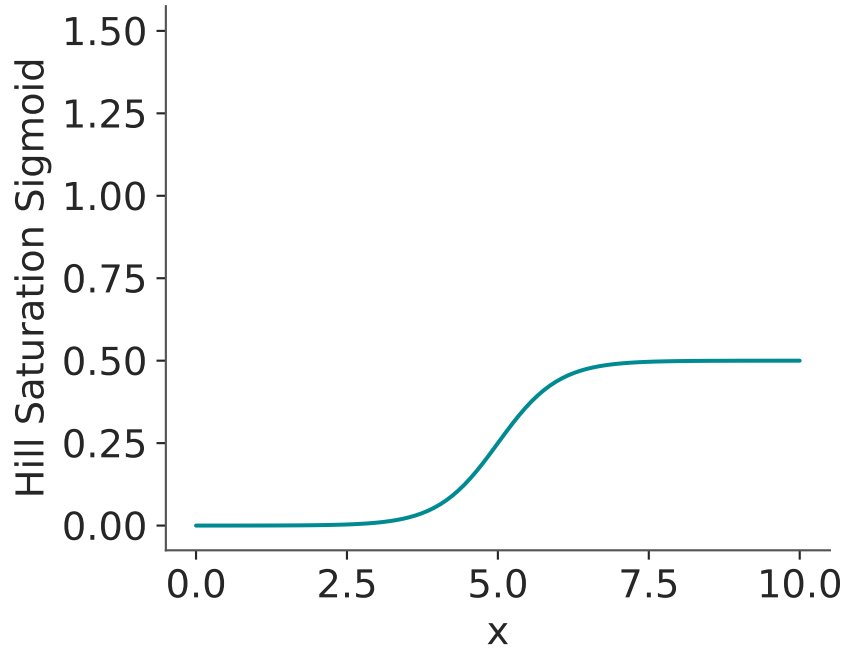
Sigma = 0.5
